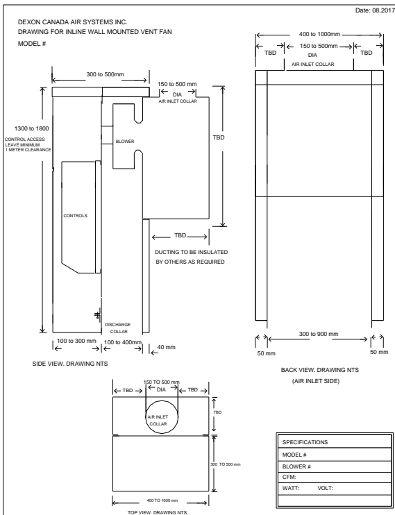
Fig. 3 – IMDH Round Inlet, Rectangle Outlet
