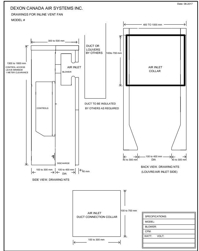
Fig.2 – IMDH Rectangle Inlet, Round Outlet
