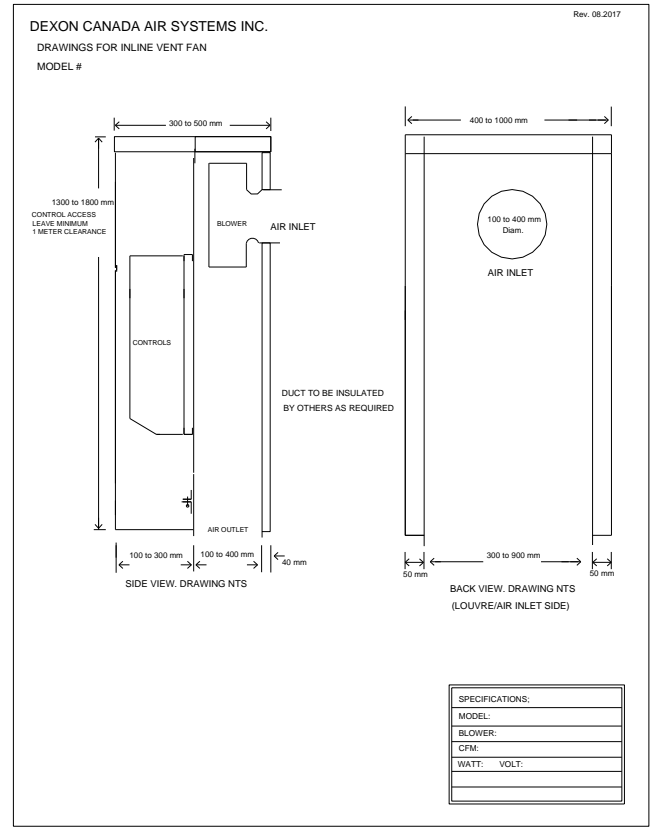
Fig.6 – IMDH Round Inlet, Rectangle Outlet
