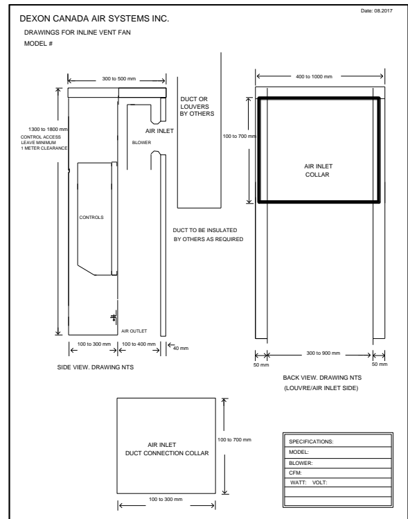
Fig.4 IMDH Rectangle Inlet, Rectangle Outlet
