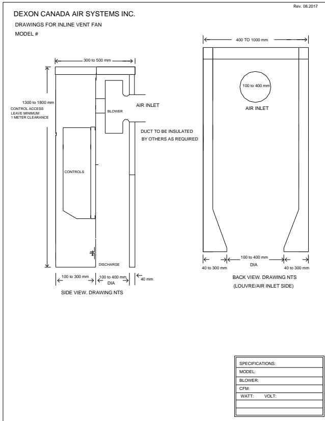
Fig. 5 – IMDH Round Inlet, Round Outlet
