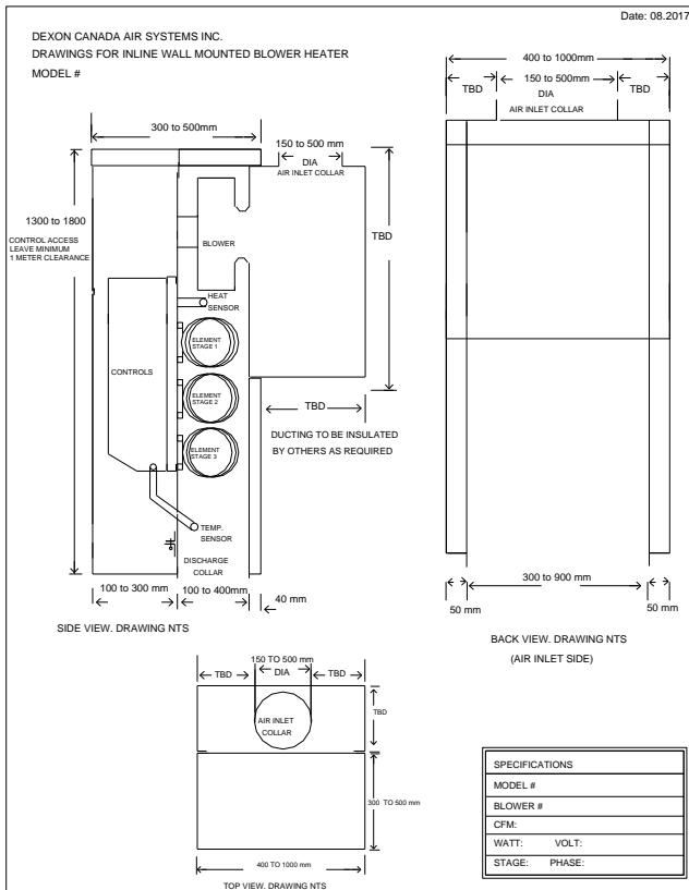
Fig. 3 – IMDH Round Inlet, Rectangle Outlet
