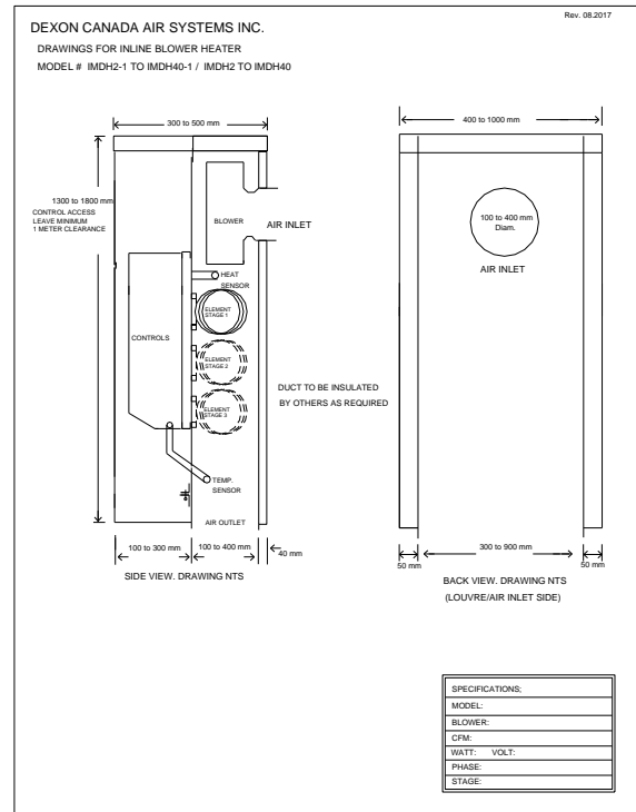
Fig.6 – IMDH Round Inlet, Rectangle Outlet
