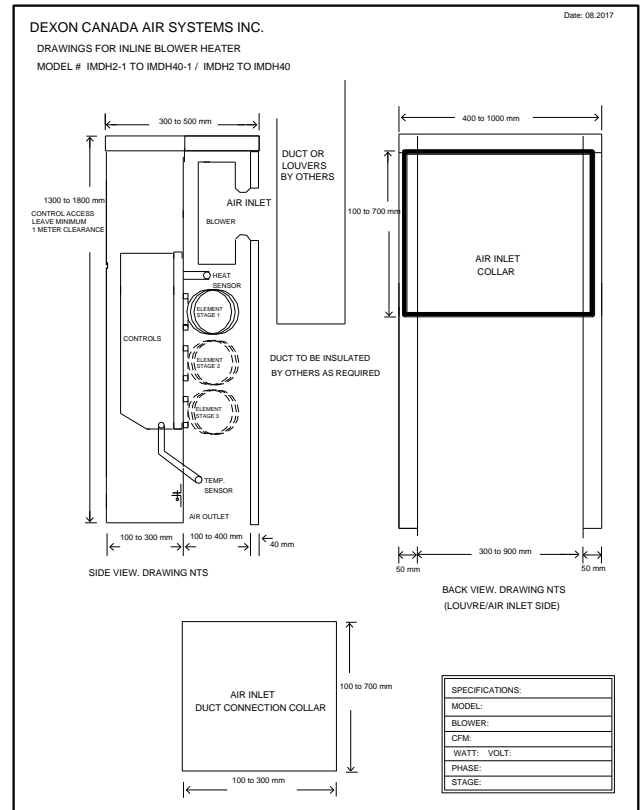
Fig.4 IMDH Rectangle Inlet, Rectangle Outlet
