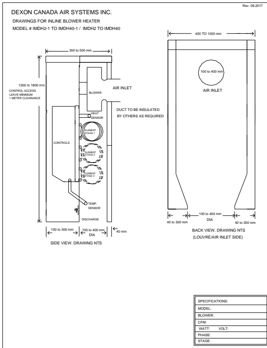
Fig. 5 – IMDH Round Inlet, Round Outlet
