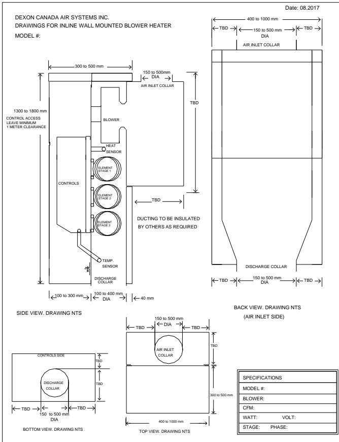
Fig. 1 – IMDH Round Inlet, Round Outlet
