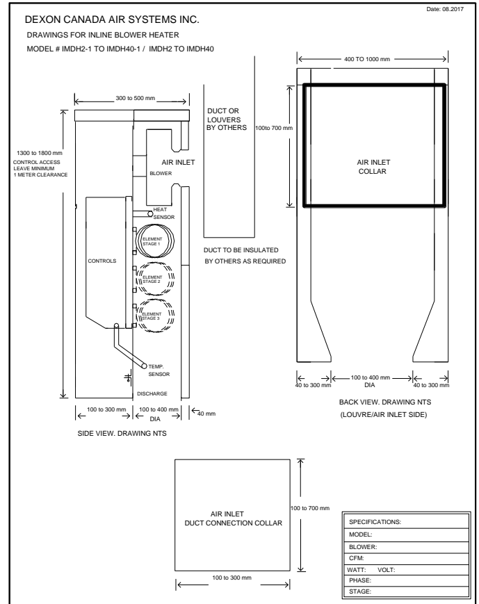
Fig.2 – IMDH Rectangle Inlet, Round Outlet
