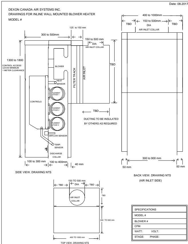
Fig. 3 – IRVDH Round Inlet, Rectangle Outlet
