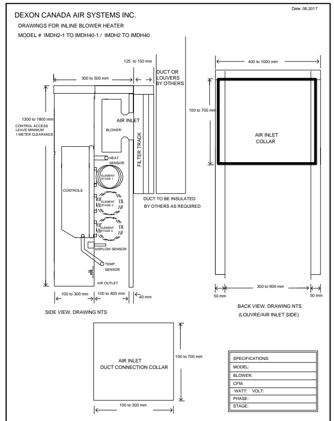
Fig.4 IRVDH Rectangle Inlet, Rectangle Outlet
