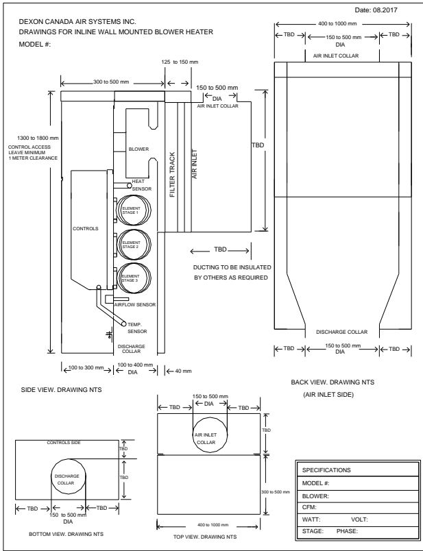
Fig. 1 – IRVDH Round Inlet, Round Outlet
