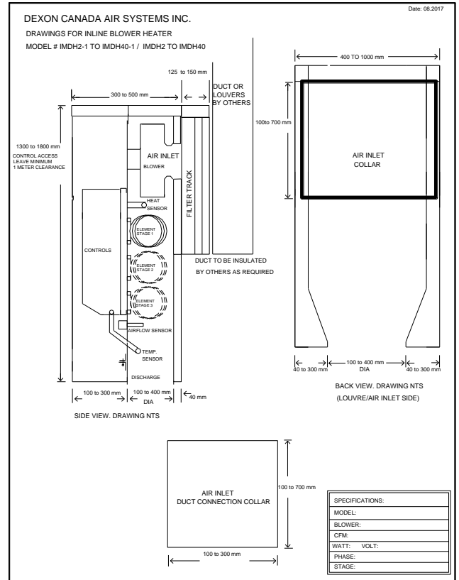
Fig.2 – IRVDH Rectangle Inlet, Round Outlet
